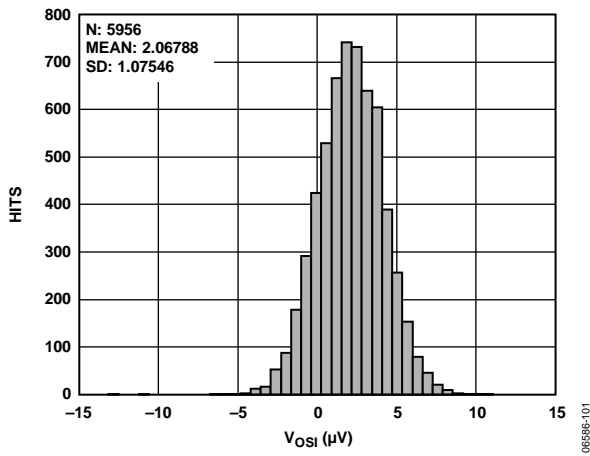
Figure 4. Instrumentation Amplifier Input Offset Voltage Distribution
